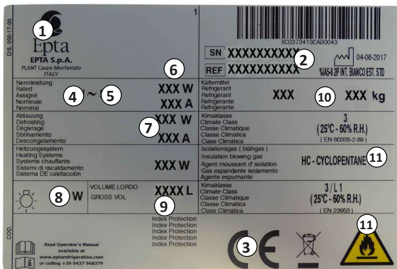
*Example of data plates
